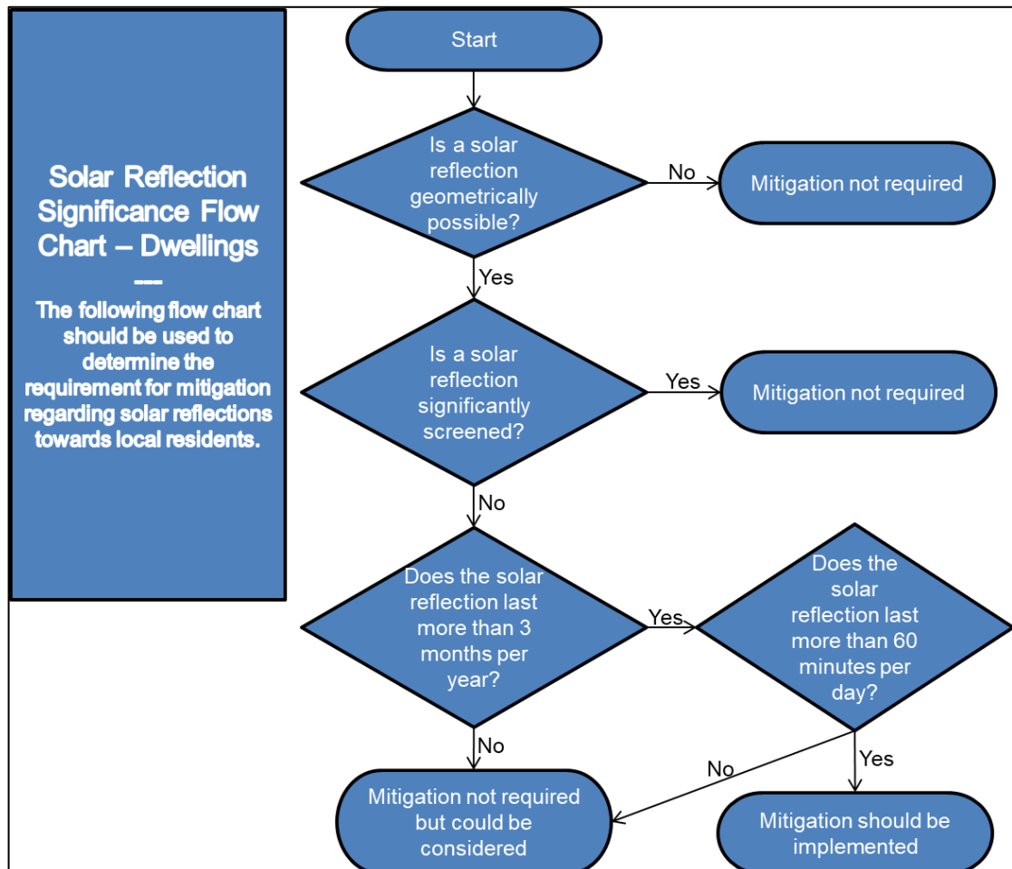
Figure 9 Dwelling impact significance flow chart
