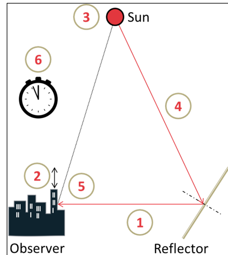
Figure 6 Conditions for determining significant glint and glare
