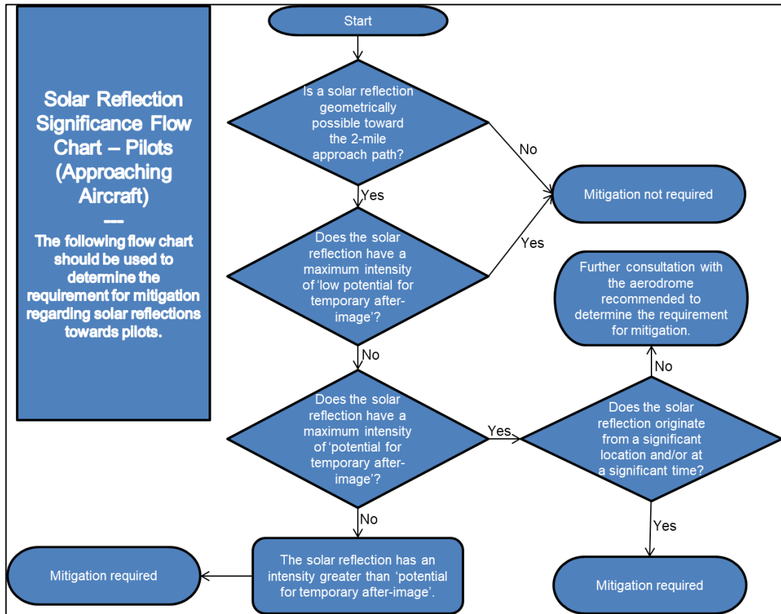
Figure 17 Pilots (approaching aircraft) impact significance flow chart
