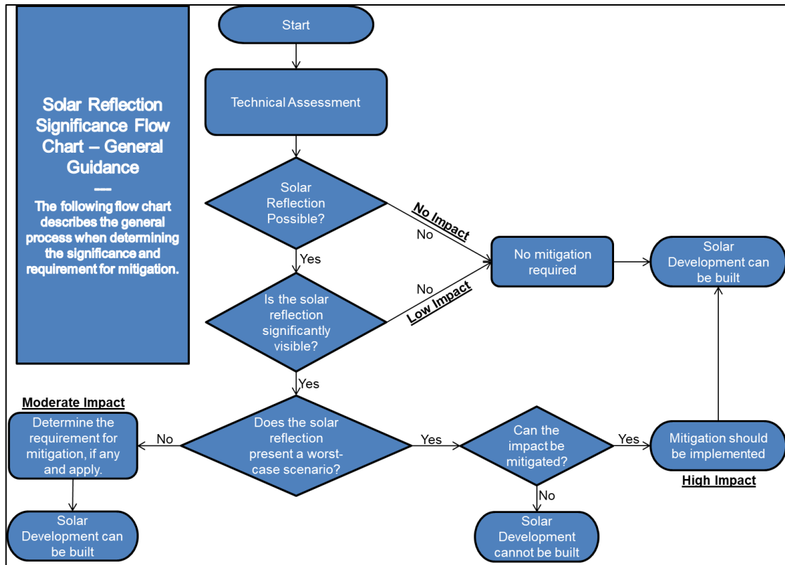
Figure 7 General process for determining the significance of glint and glare
