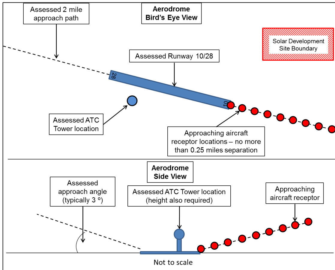
Figure 15 Illustration showing receptor identification process – aviation
