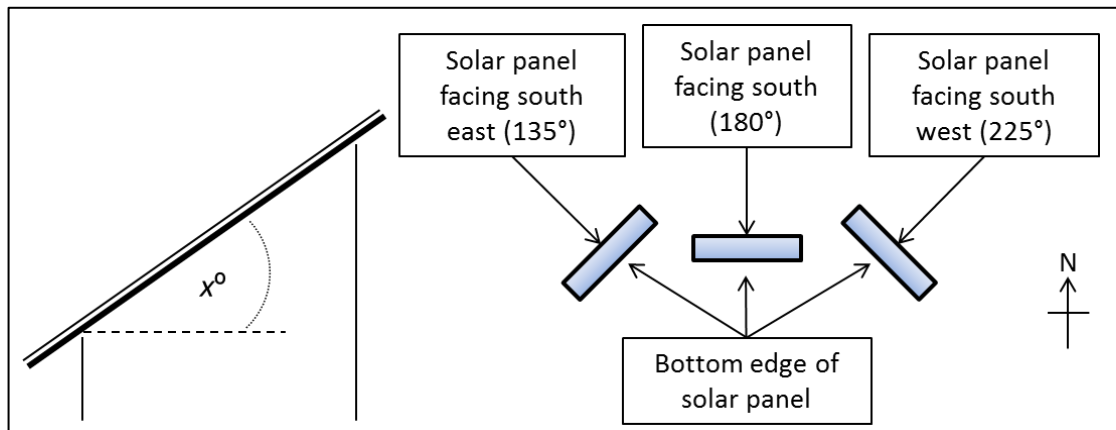
Figure 5 Illustration showing panel elevation angle (side-on) and panel azimuth angle (top down)
