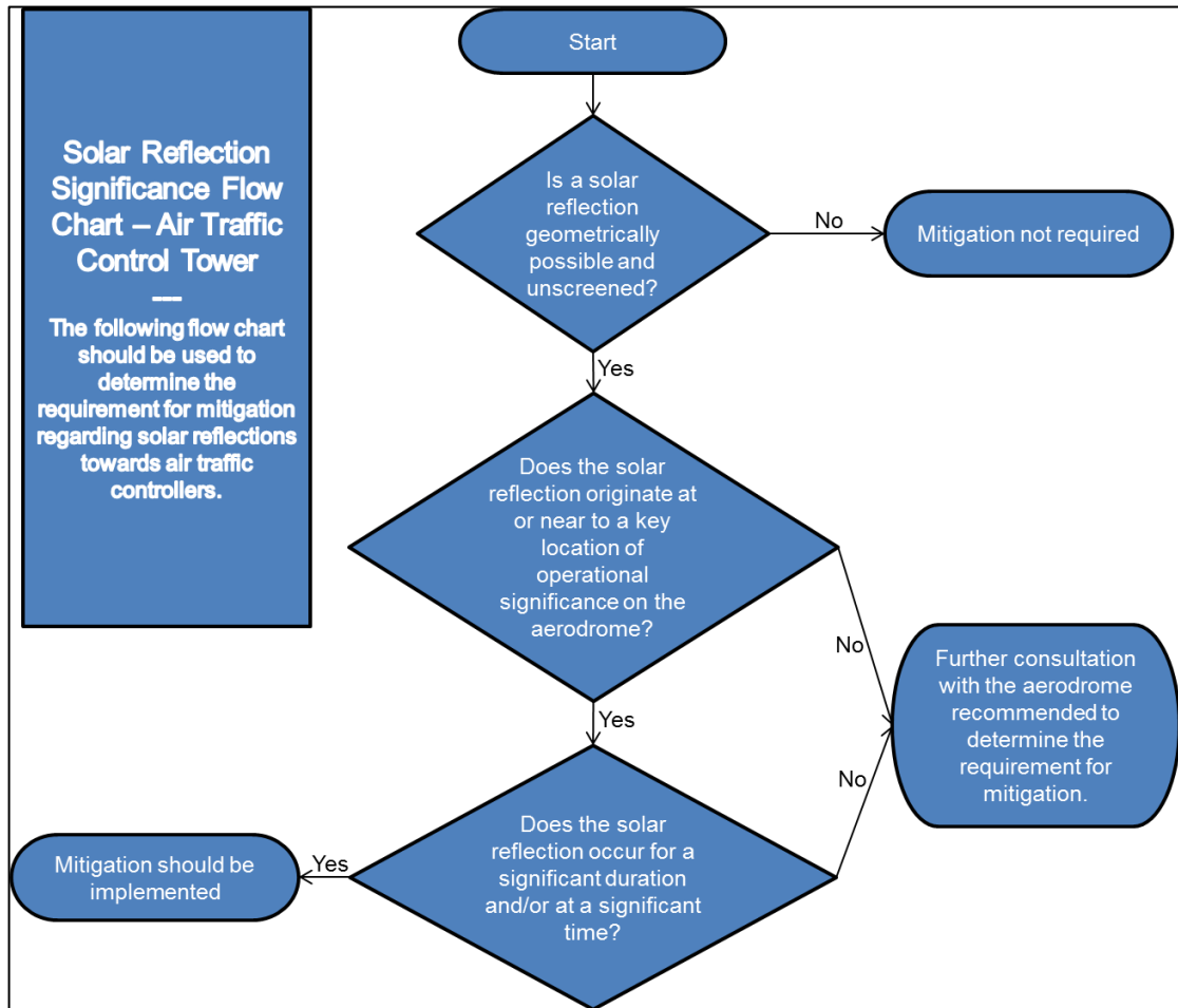
Figure 16 ATC tower impact significance flow chart
