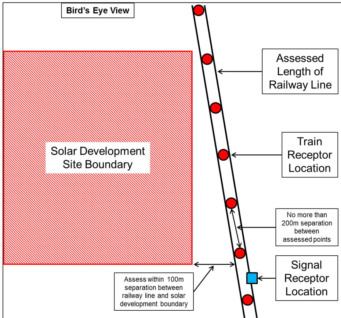
Figure 13 Illustration showing receptor identification process – train drivers and signals
