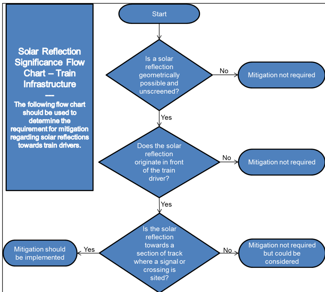
Figure 14 Train driver impact significance flow chart
